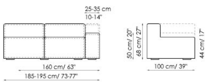
Terminale 185/195 End section Prof.100 dx depth right
