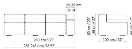
Terminale 235/245 End section Prof. 100 dx depth right
